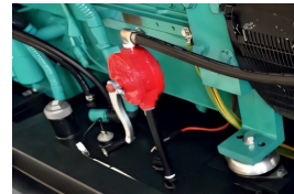
Manuelle Kraftstoff-Transferpumpe Manual fuel transfer pump
